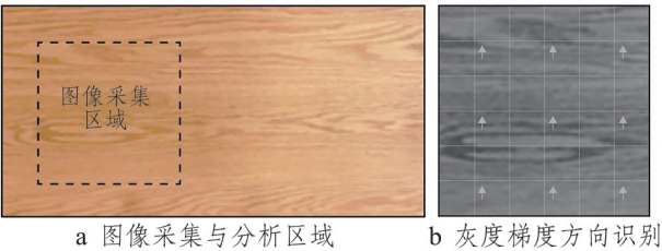
图2 基于灰度梯度分析的木材纹理方向量化原理示意 Fig.2 Schematic illustration of wood grain orientation quantification based on grayscale gradient analysis
