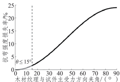
图4 木材纹理-力学性能映射模型的强度损失率曲线 Fig.4 Strength loss rate curve of mapping model of wood grain-mechanical properties
