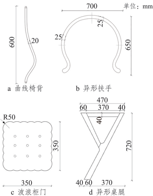
图1 家具异形零部件的4种典型轮廓类型 Fig.1 Four typical profile types of furniture irregular components
